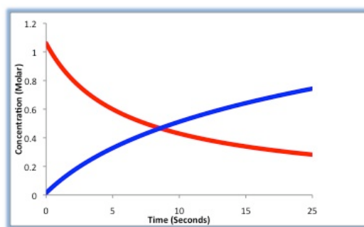
Figure 1. The above picture shows a hypothetical reaction profile in which the reactants (red) decrease in concentration as the products increase in concentration (blue).
